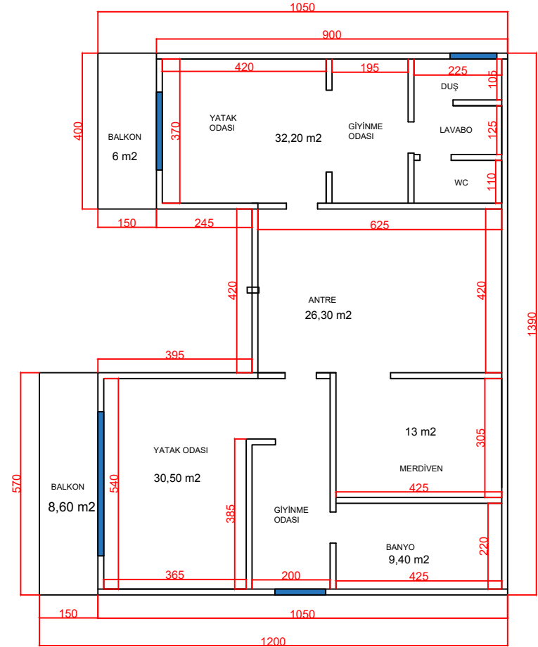
1. KAT PLANI Brüt :139 m 2
