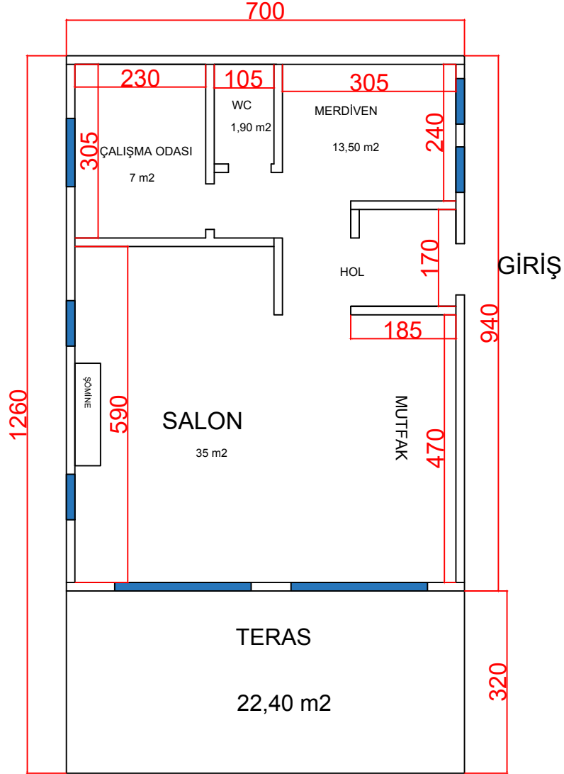
ZEMİN KAT PLANI Brüt :88 m2
