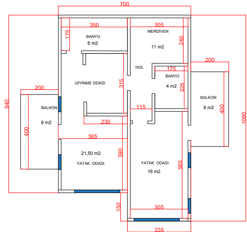
1. KAT PLANI Brüt :79 m2
