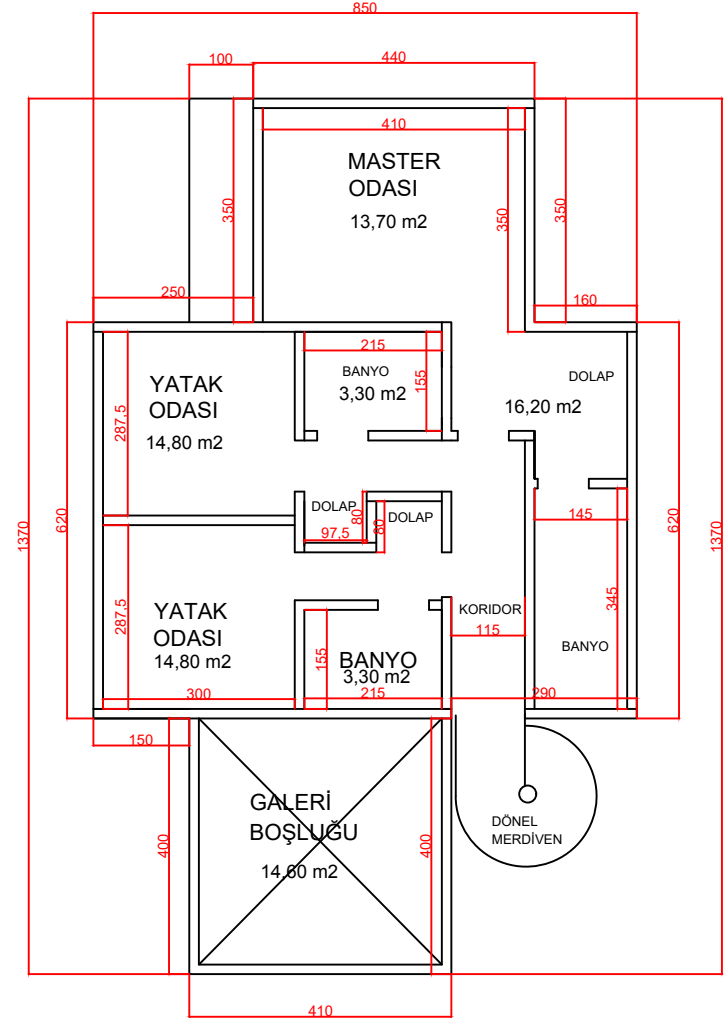
1 KAT PLANI Brüt :85 m2
