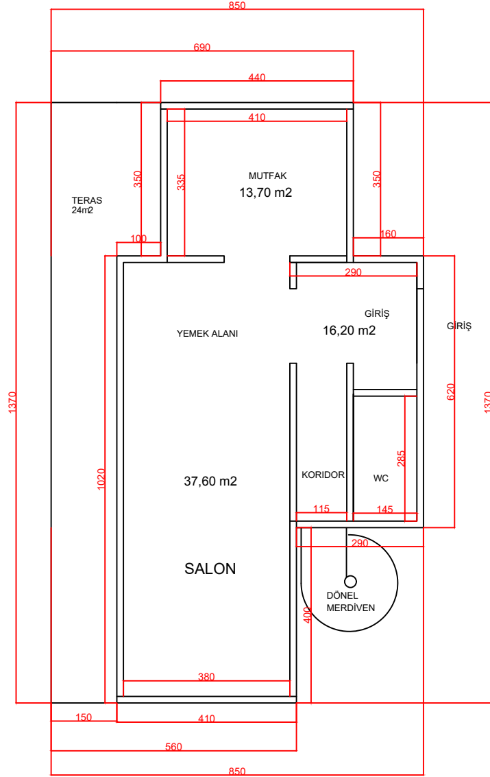
ZEMİN KAT PLANI Brüt :100 m2
